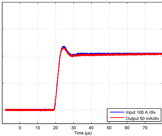
Figure 2: Typical step response (0 to 200 A, 75 A/μs R_M = 10 \Omega )
